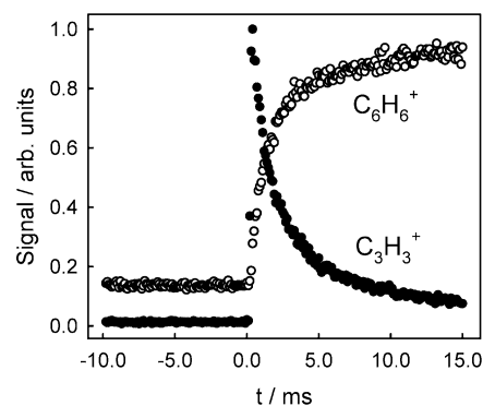
Figure 7. Typical temporal ion signal profiles of \text{C}_3\text{H}_3 and \text{C}_6\text{H}_6 recorded in an experiment to study the products of the \text{C}_3\text{H}_3 + \text{C}_3\text{H}_3 reaction. T = 1000 K, bath gas density is 6.0 \times 10^{16} , [\text{C}_3\text{H}_4] = 4.62 \times 10^{15} , [(\text{CClO})_2] = 1.68 \times 10^{15} , and [\text{C}_3\text{H}_3]_0 = 1.12 \times 10^{13} molecules \text{cm}^{-3} .
