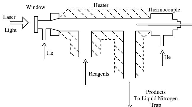
Figure 2. Reactor constructed for the study of the final products of the self-reaction of propargyl radicals.
