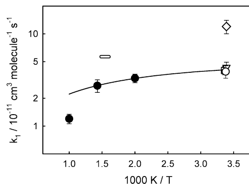
Figure 6. Temperature dependence of the experimentally obtained values of k_1 (filled circles). Diamond, inverted triangle, square, open circle, and short white line represent the values of k_1 reported in refs 10, 11, 5, 13 and 4, respectively. The solid line represents the fit of eq II.
